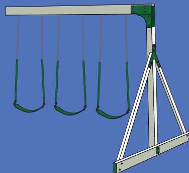
3 POSITION SINGLE BEAM
